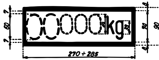
Figure 2: Wagon tare and braked weight of the platform-operated hand brake
