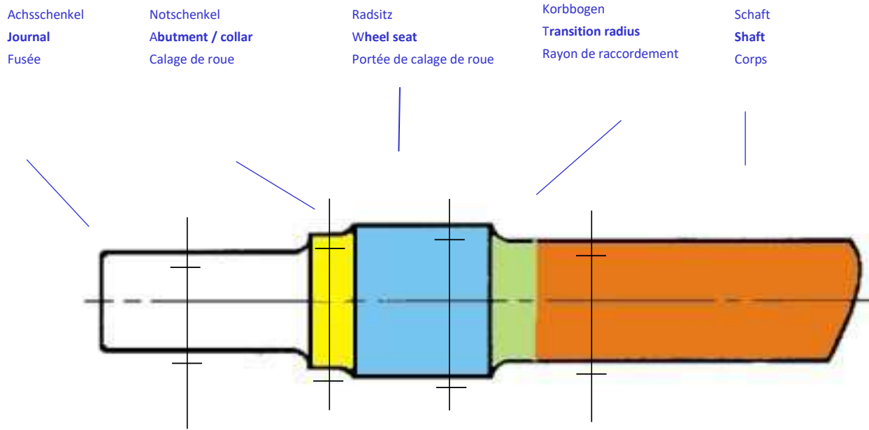
Axle
