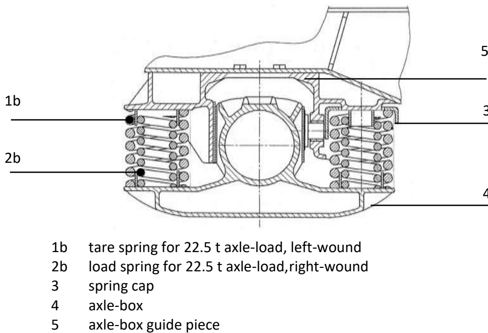
Figure 2 – Bogie with springs for axle-load of 22.5 tonnes
