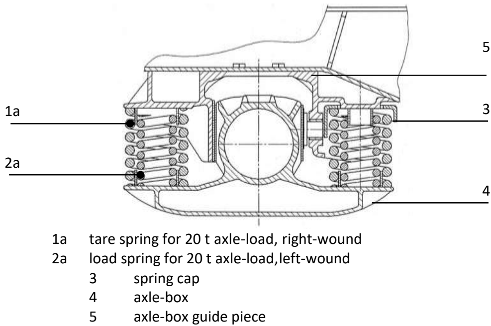
Figure 1 – Bogie with springs for axle-load of 20 tonnes
