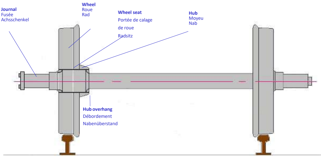
Wheelset
