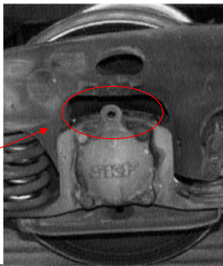
Fig. 7: Manganese wear plates on bogies and axle-boxes detached
