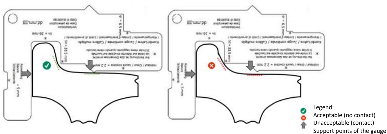
Fig. 7 – Projection
