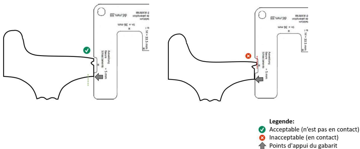
Figure 8 : Faux boudin
